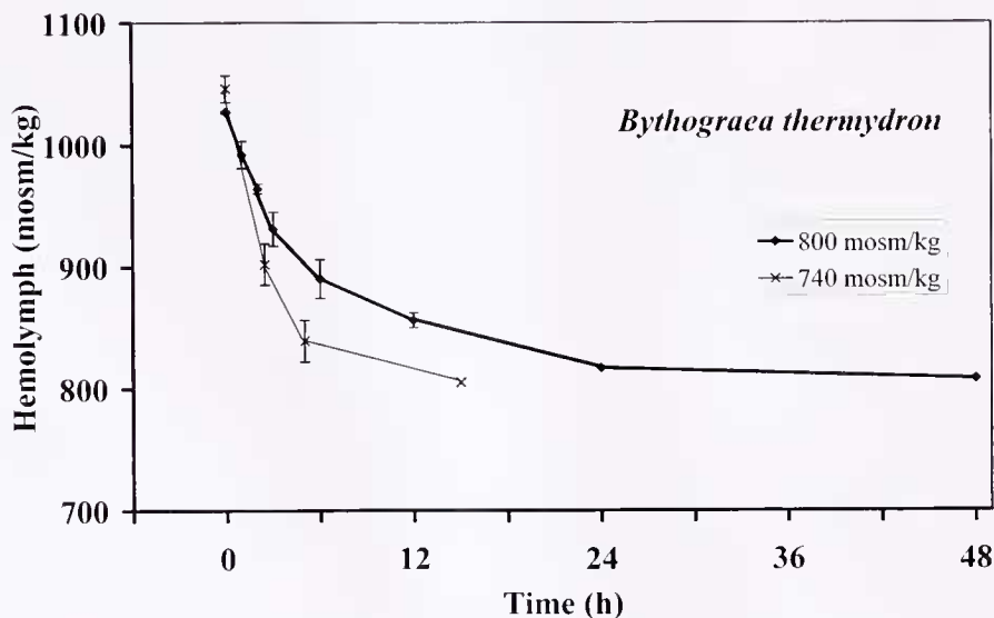
Figure 2. Bythograea thermydron . Change in hemolymph osmolality according to the time after rapid transfer from Pacific surface seawater ( 1002 \pm 2 mosm/kg) to dilute media at 740 mosm/kg and 800 mosm/kg. Error bars: mean \pm SD, n : 4 to 6 individuals.
